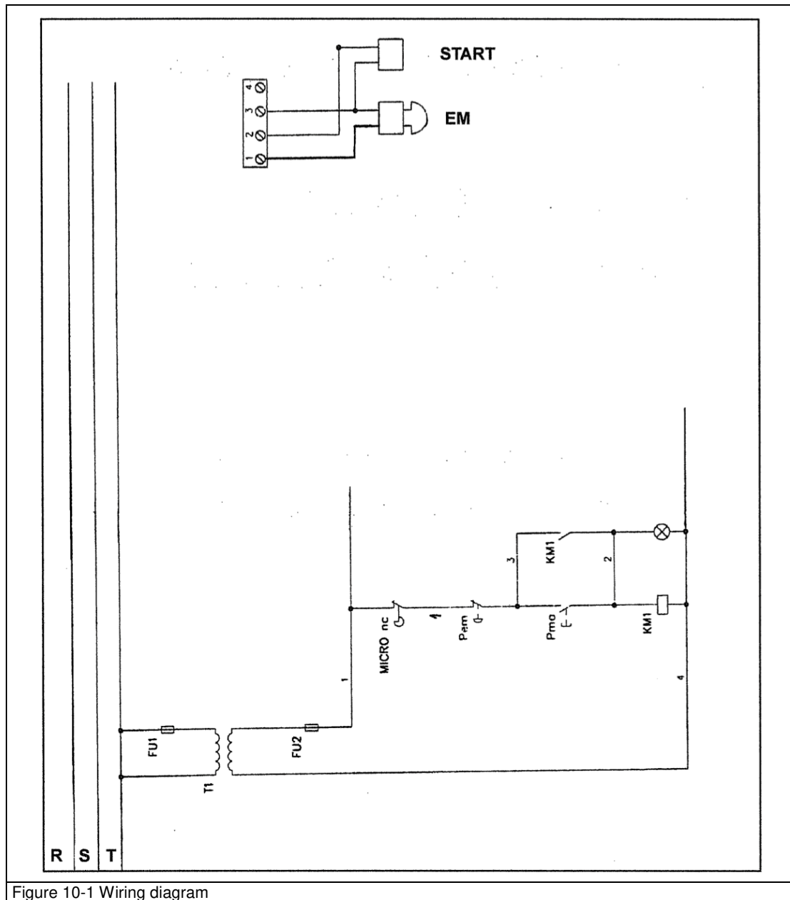
Figure 10-1 Wiring diagram
